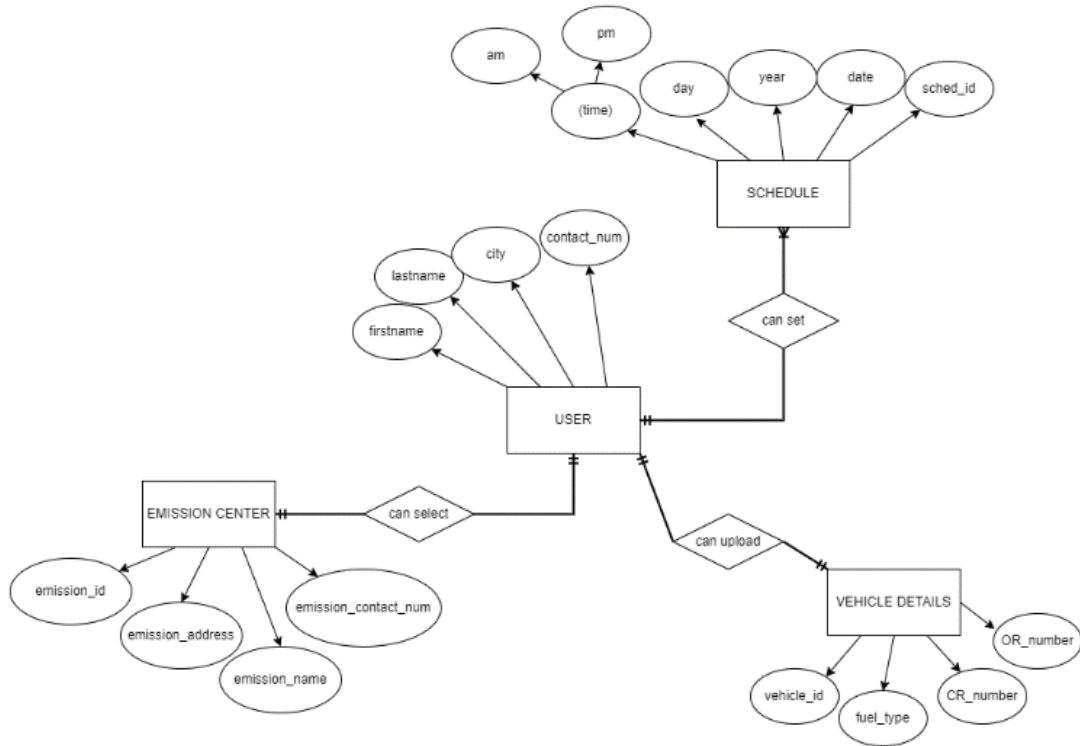
Figure 4. Entity-Relationship Diagram
